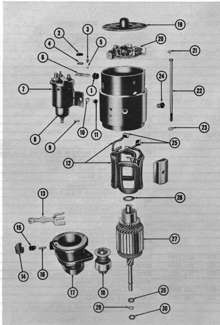
STARTING MOTOR 163 80
