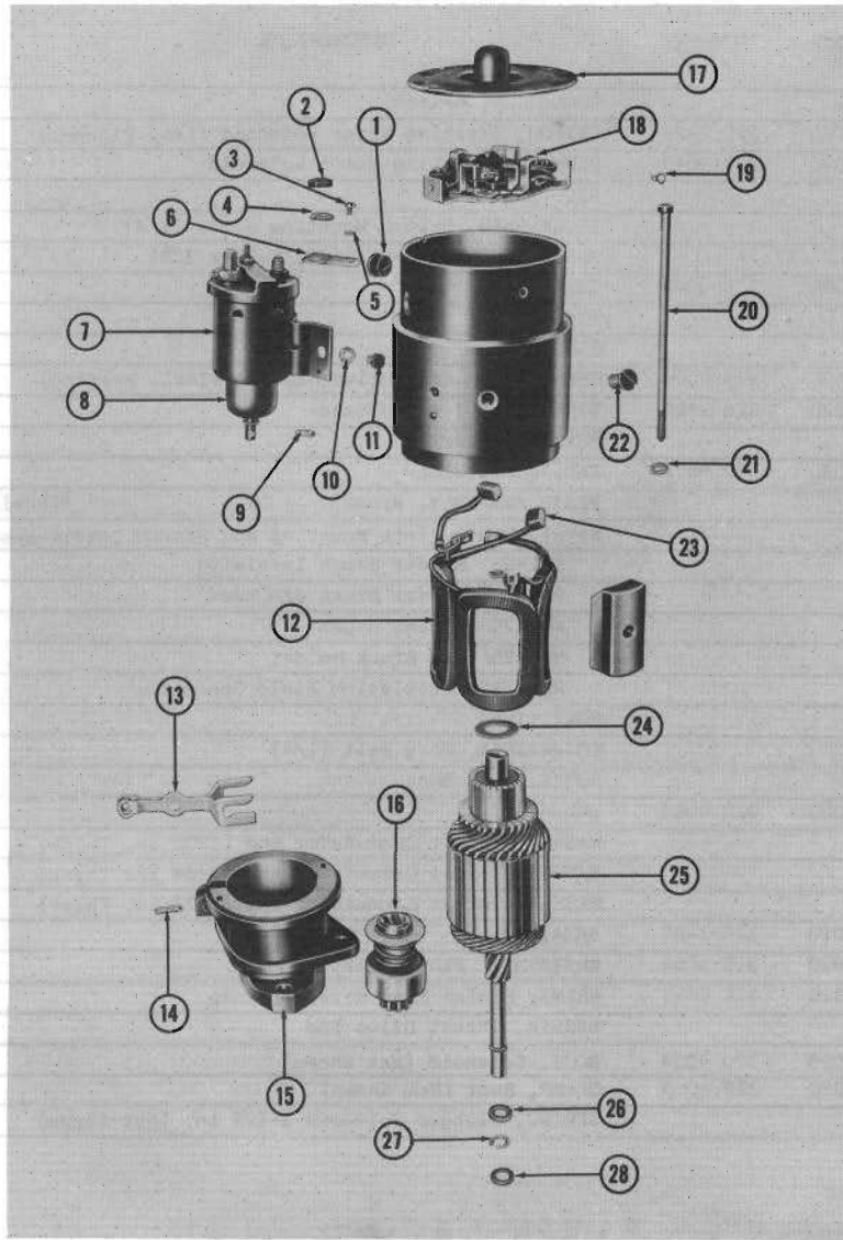
STARTING MOTOR 162-163 01-10
