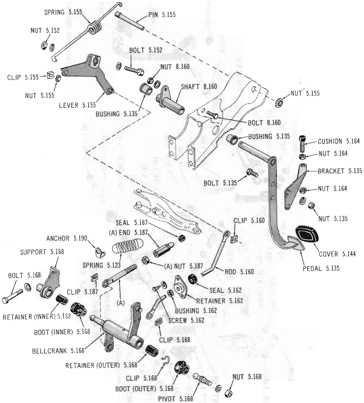
(A) Part of LINK ASSY. 5.187
