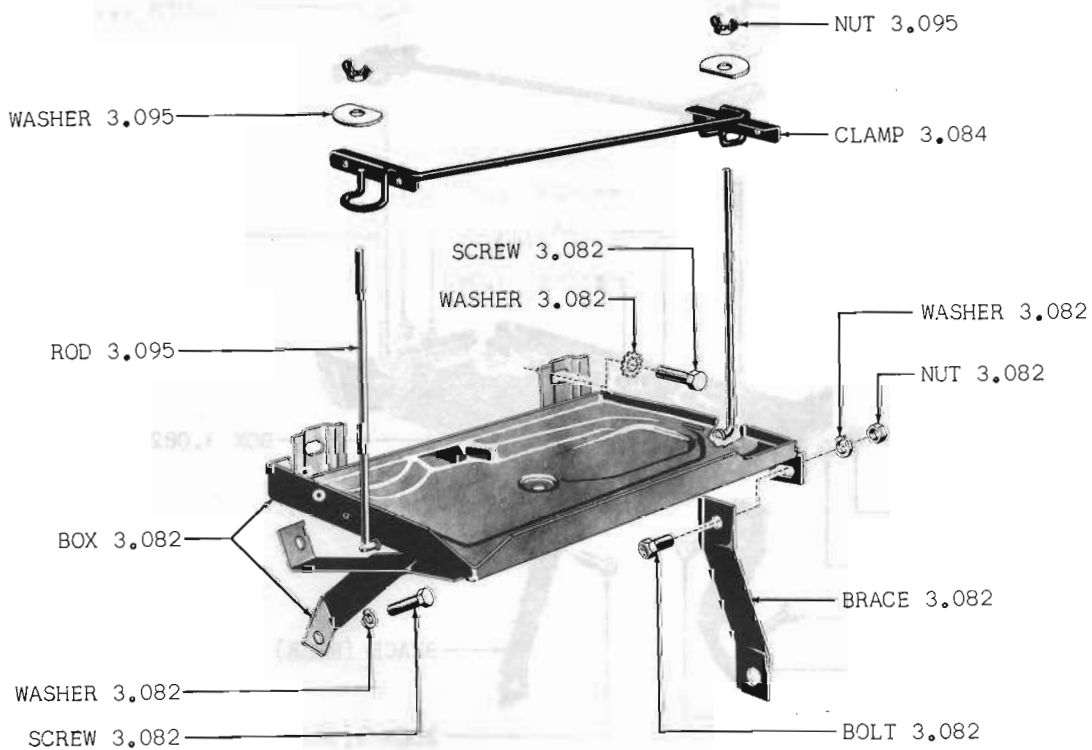
BATTERY BOX 60-61 80
