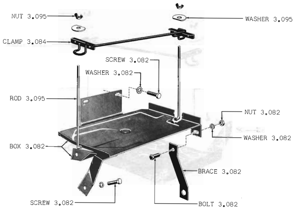
BATTERY BOX 60-61 20
