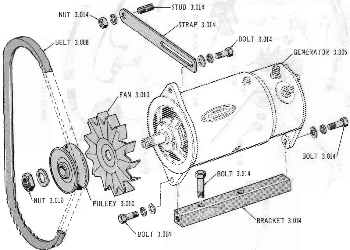
GENERATOR FAN, PULLEY AND MOUNTING 63-64 01 (LAC)
