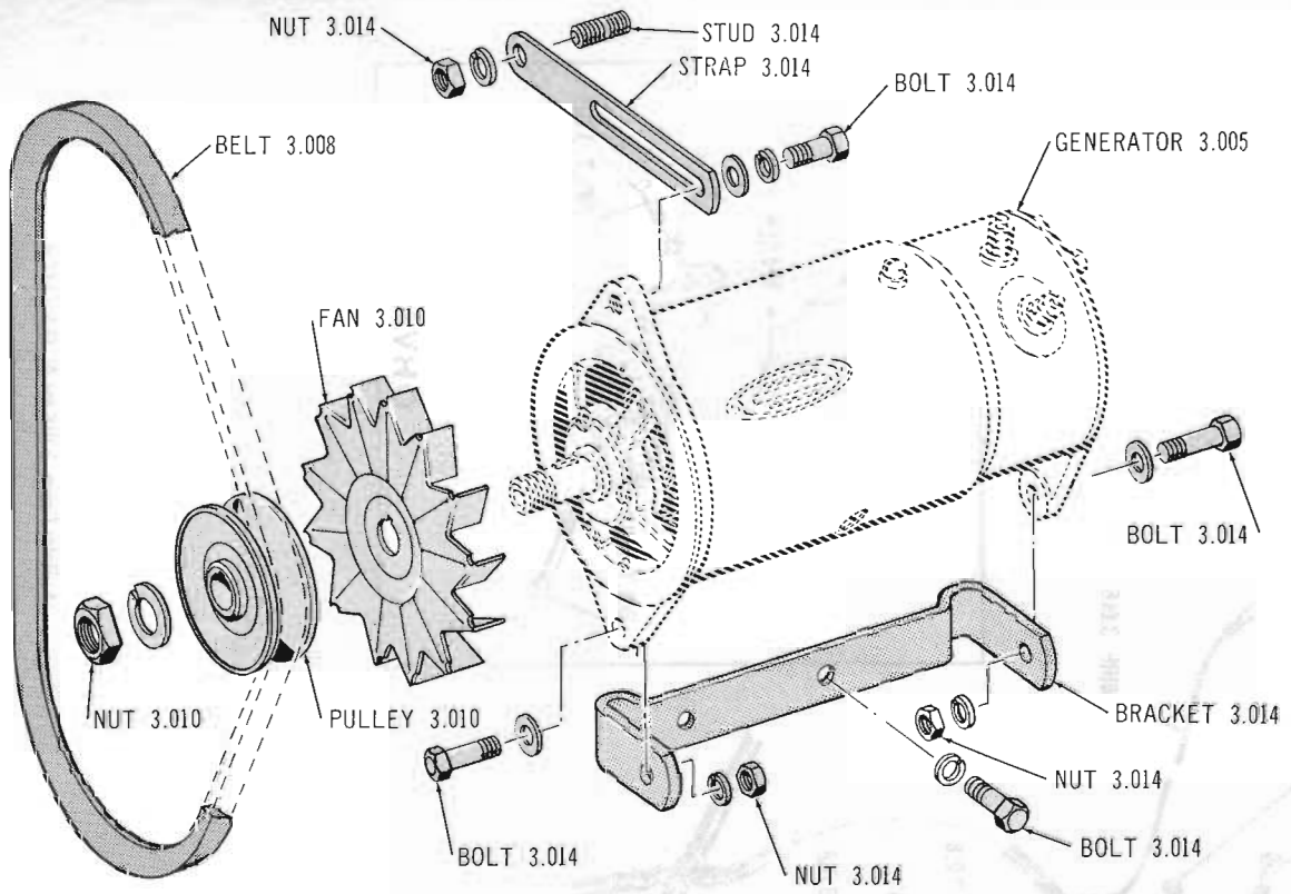
GENERATOR FAN, PULLEY AND MOUNTING 63-10 (LAC)
