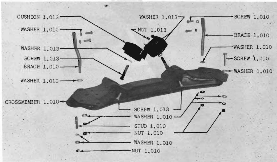
ENGINE REAR SUPPORT 60 thru 62 20-80
