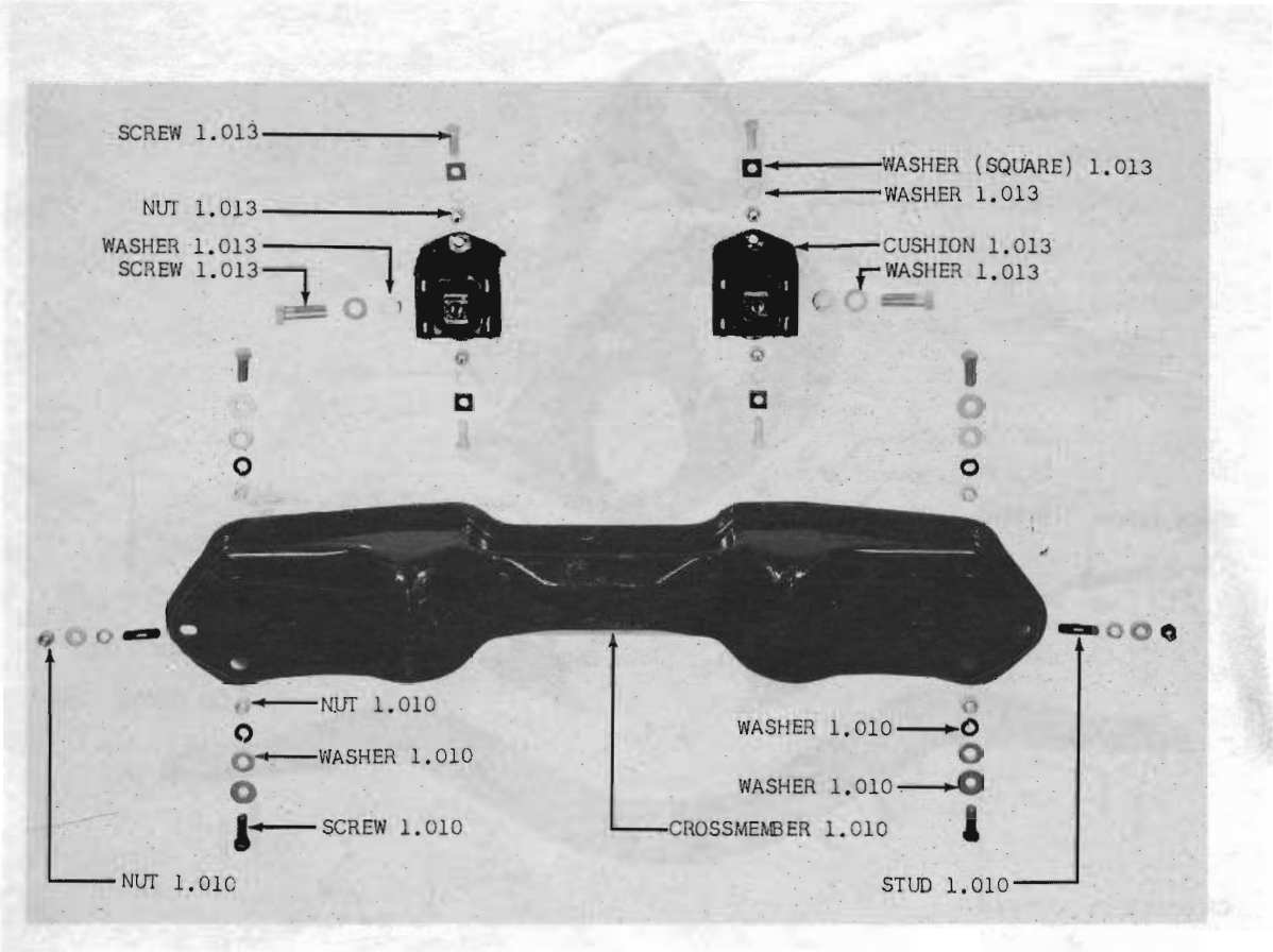
ENGINE REAR SUPPORT 60 thru 62 10
