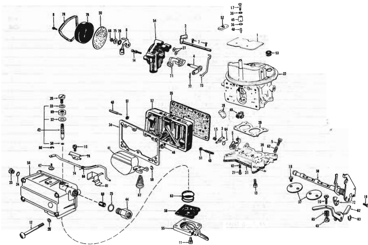
CARBURETOR 61 20-80 (DUAL THROAT)
