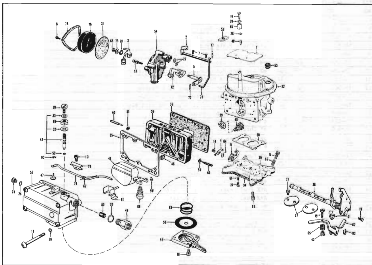
CARBURETOR 60 20-80 (Dual Throat)
