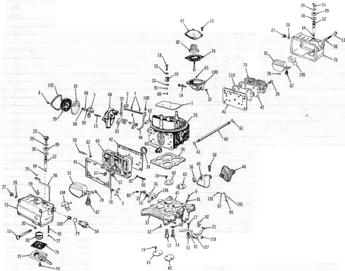
CARBURETOR 65 10-80 (V8-W4B)
