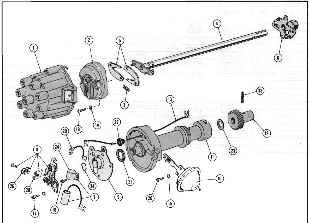
DISTRIBUTOR 63 Thru 65 10-80 (V8)
