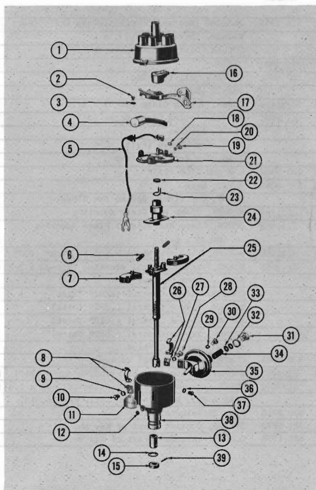
DISTRIBUTOR 62 01 (LHE)
