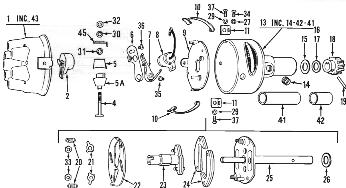
DISTRIBUTOR 60-61 01-10 (OHV)
