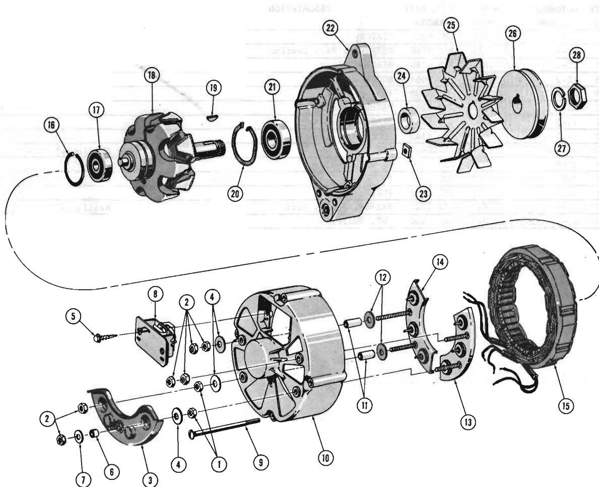
ALTERNATOR (Less Pulley and Belt)(55 AMP.) 64-65 01-10-80
